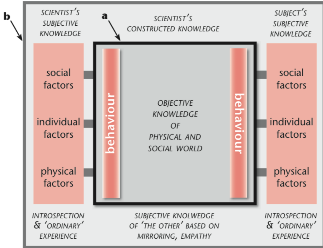
Figure 3. Constructionism
